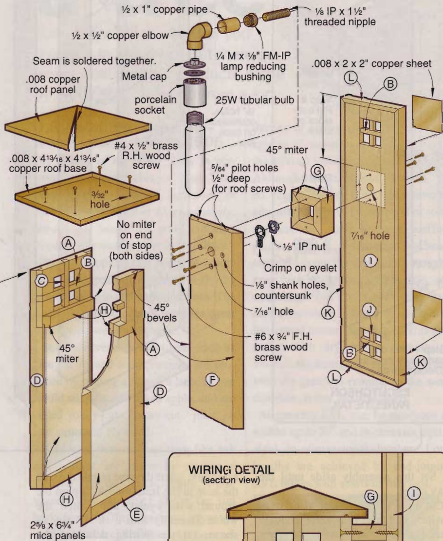
EXPLODED VIEW
